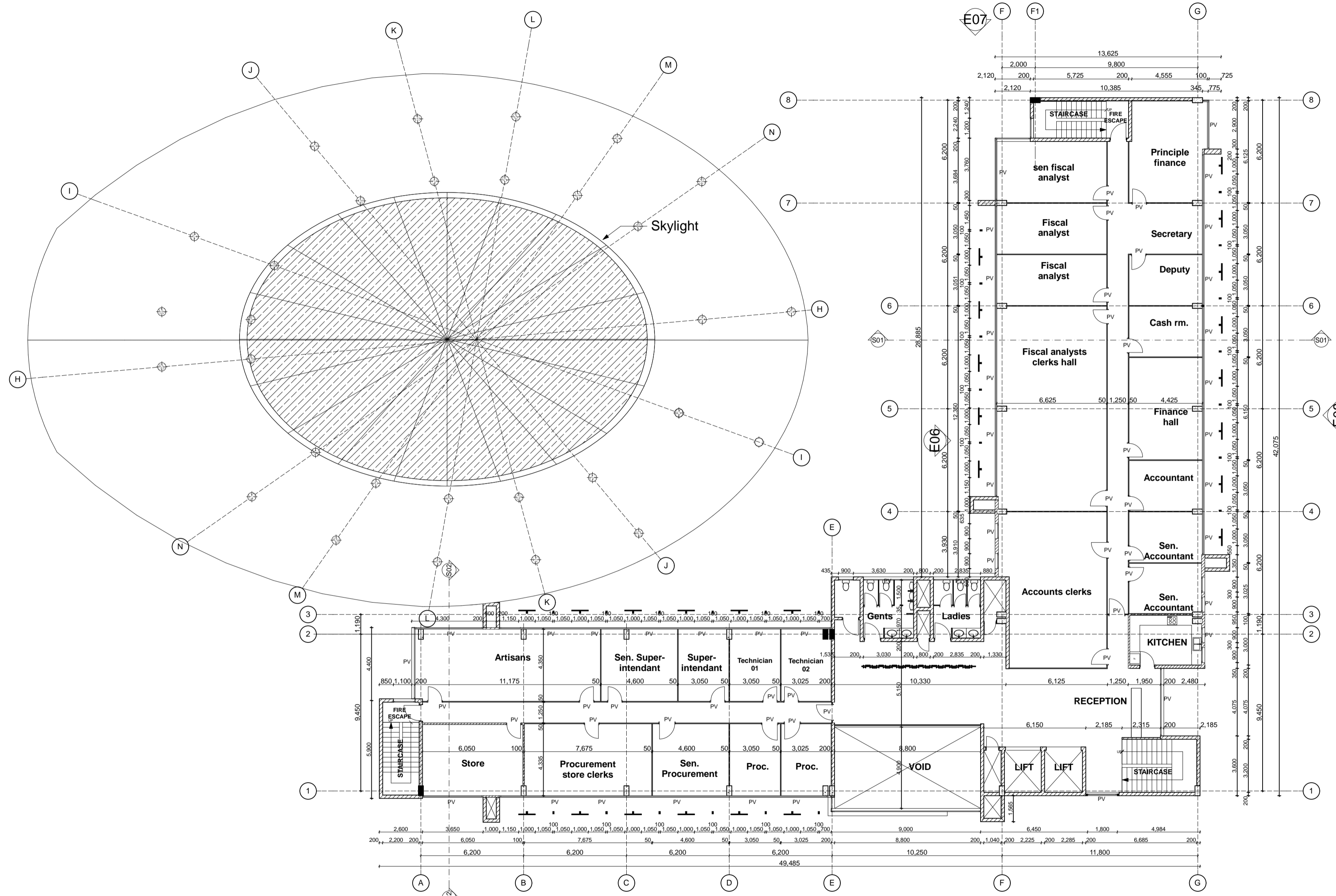
THIRD FLOOR (Scale 1:125)
