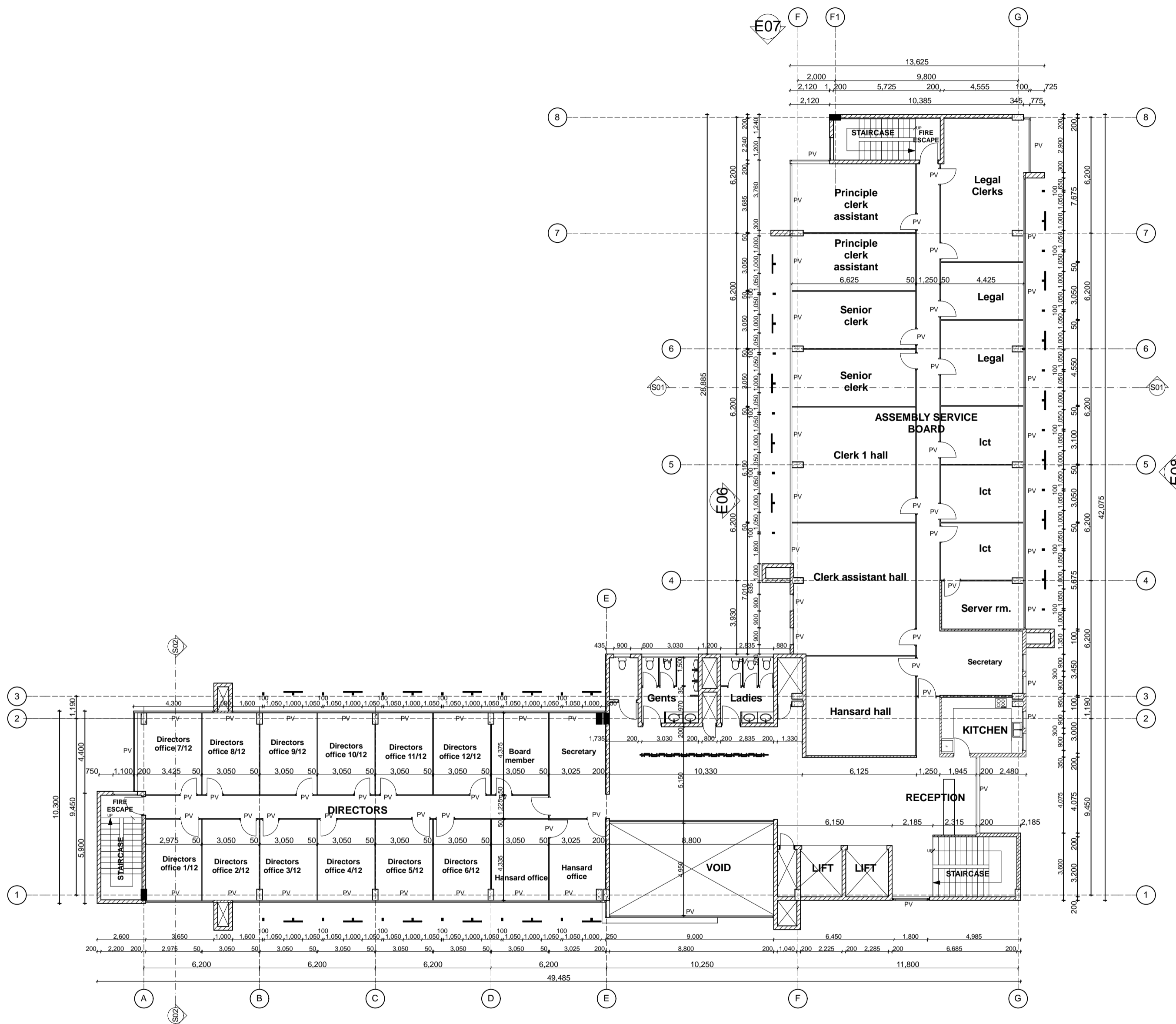
FOURTH FLOOR (Scale 1:125)
